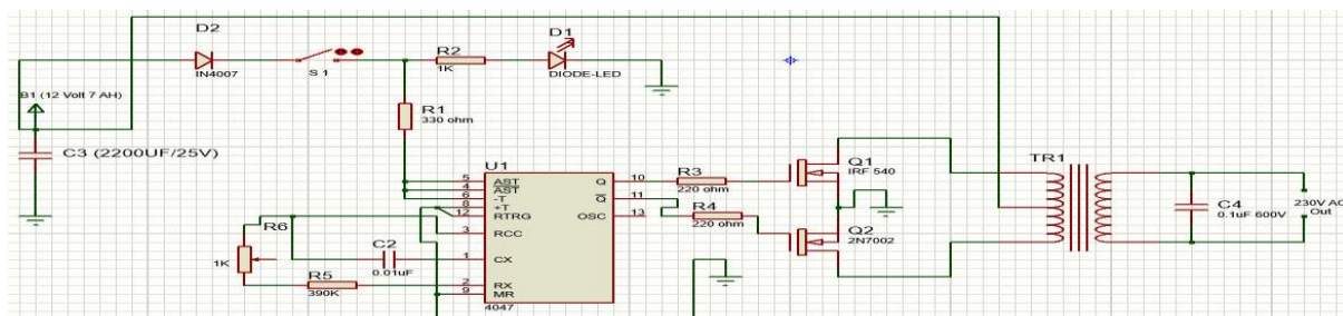
Fig. 7: Circuit Diagram of the Power Inverter drawn in Proteus ISI
